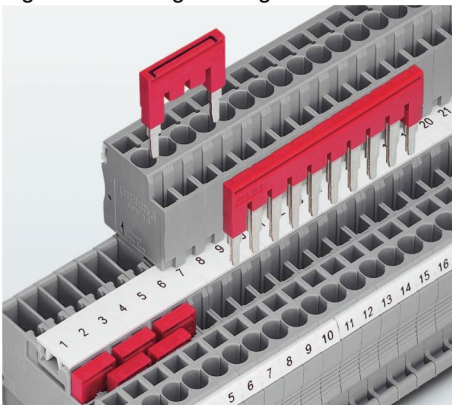
Figure 8 Plug-in bridges
